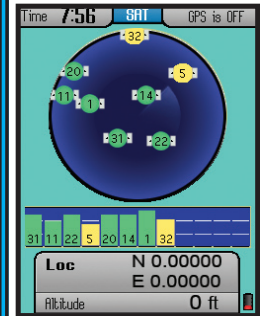
Fig 25. SAT Page
